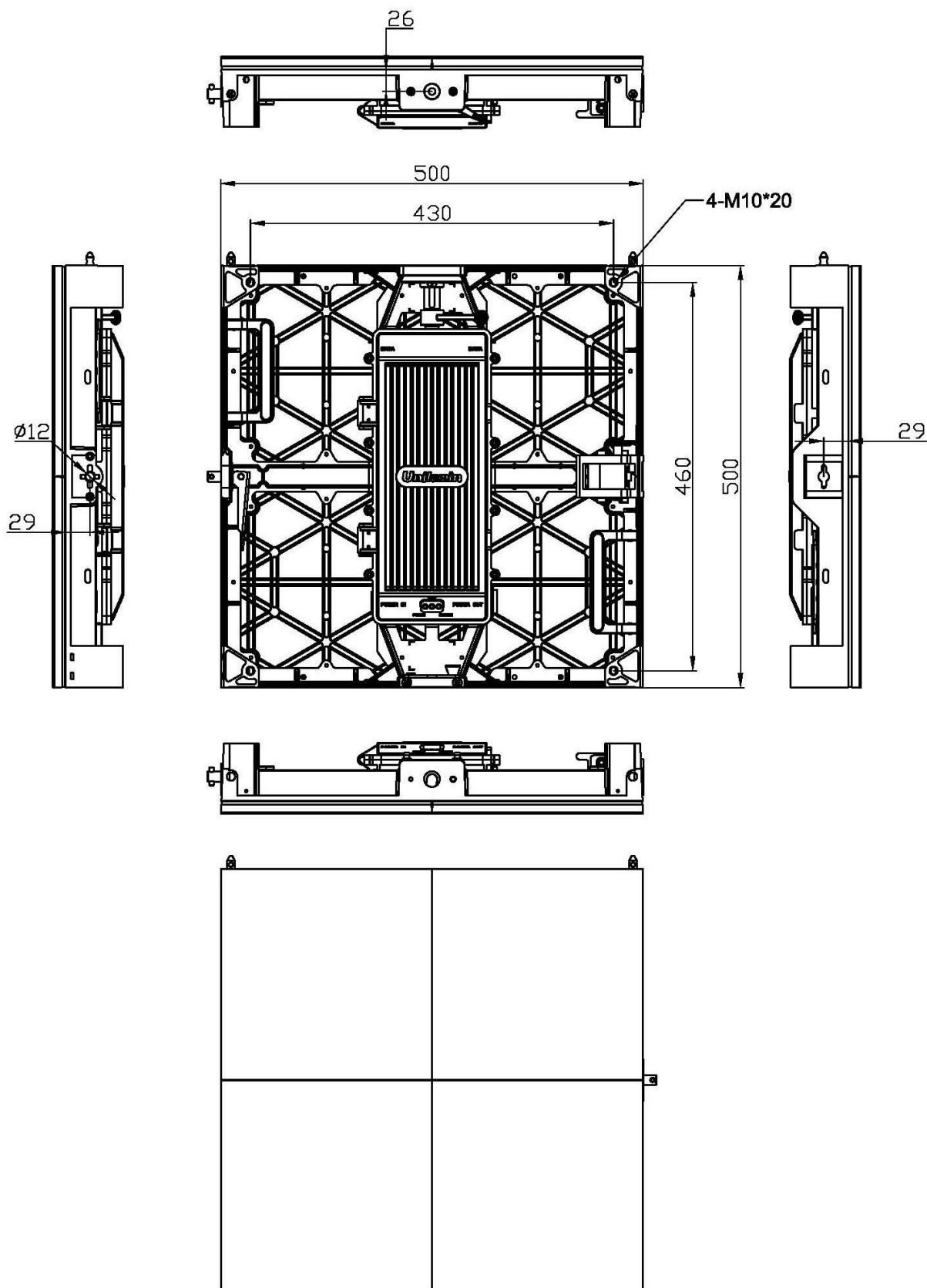
Fig1. Cabinet Dimension
